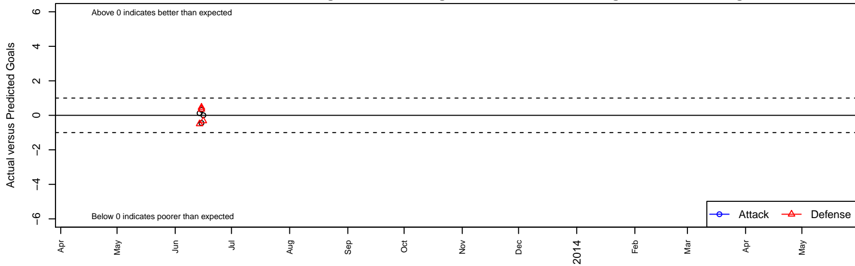
CUSA Oregon Fires B01 Dots are actual minus expected GF (blue circles) and GA (red triangles). Blue line is smoothed change in attack strength. Red is smoothed change in defense strength.
